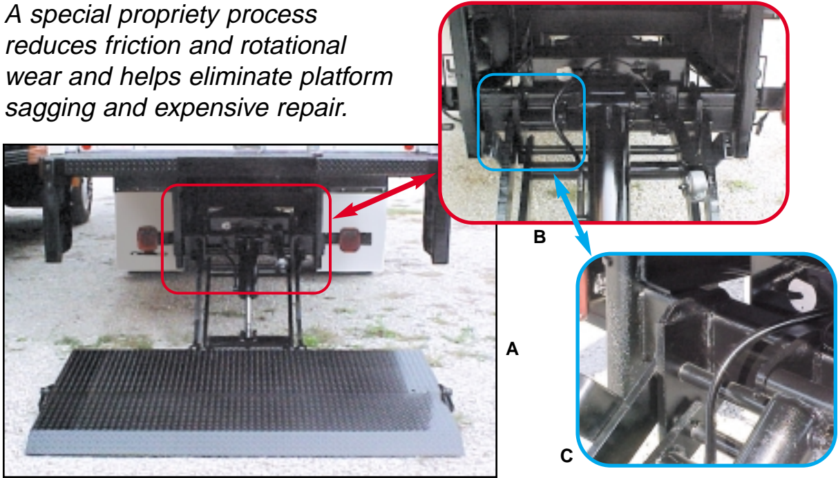
Three views of the ATU Tuckunder liftgate (A), Adapter frame assembly area (B), and closeup of the adapter frame and pin (C).
