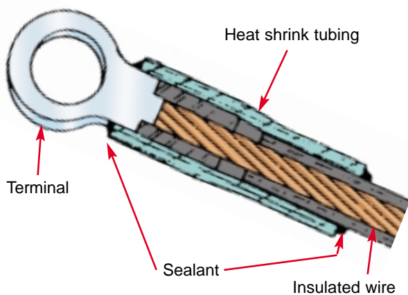
Cut-away section of Anthony heat shrink terminal connection
